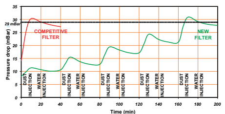
Alternative Wet/Dry Dust Holding Capacity
