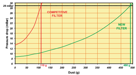
Dust Holding Capacity with Carbon Black at 700 g/s
