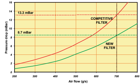
Pressure Drop with New Filters
