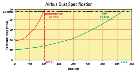
Dust Holding Capacity with Spec at 700 g/s
