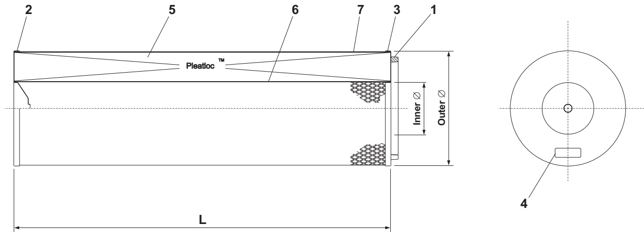
DIN top flange Closed bottom end cap with Ø13.5 mm hole
