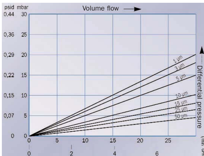
Flow rate of a 10" PP-TF element – water
