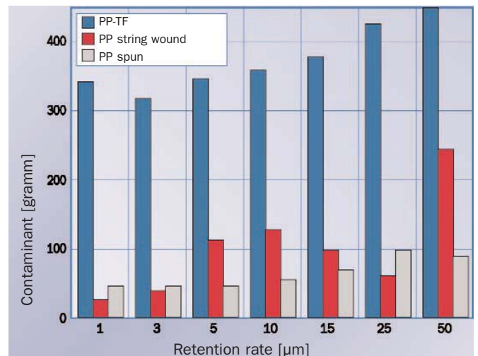
Dirt hold capacity Ultrapolydepth
