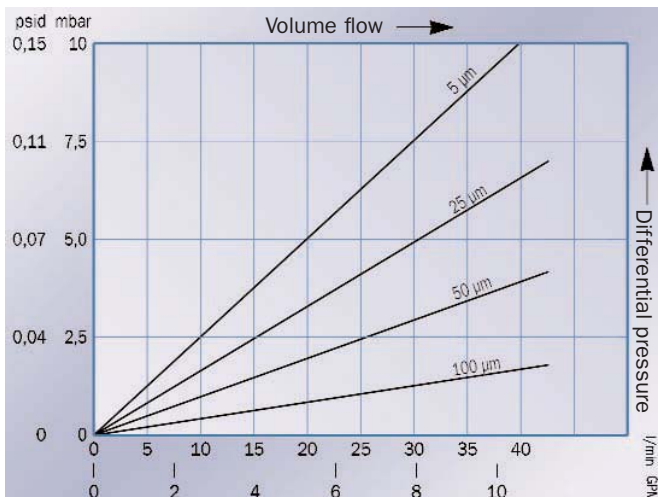
Flow rate of a 10" P-SM element – water
