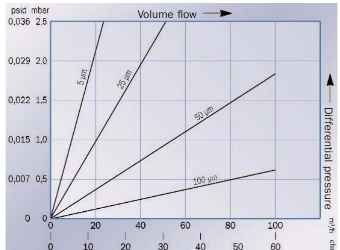
Flow rate of a 10" P-SM element – air
