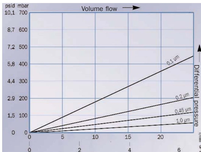
Flow rate of a 10" P-PF-PT elements – water (1 bar, 20°C)
