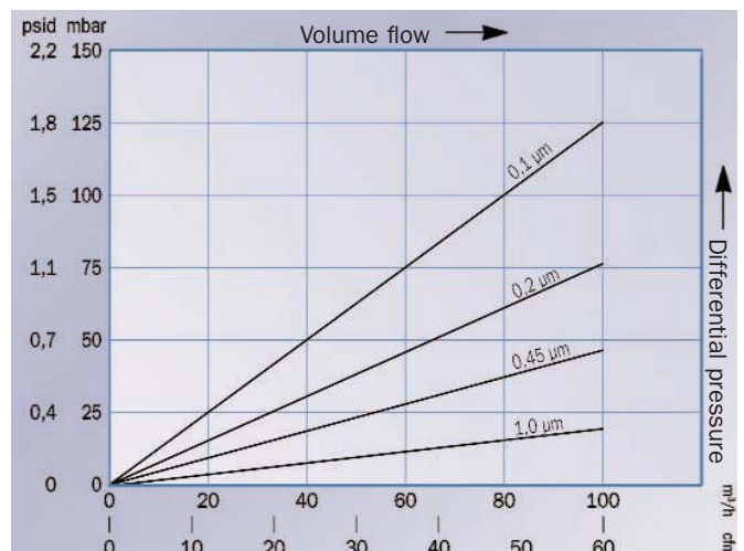
Flow rate of a 10" P-PF-PT elements – air (1 bar, 20°C)
